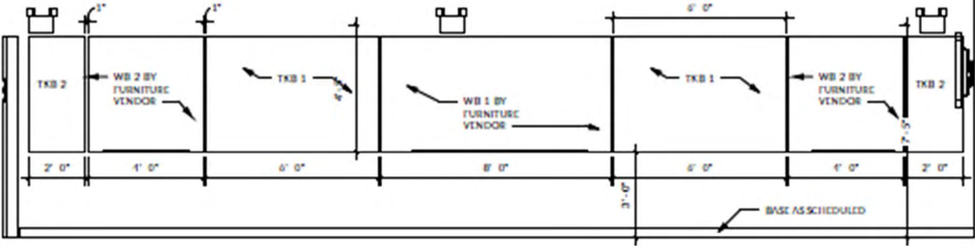
10 LARGE MEETING ROOM WEST WALL A302 3/8\"/>
